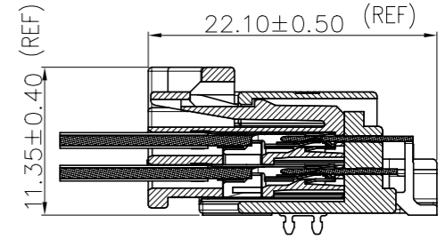
Housing and Wafer Assembly drawing
