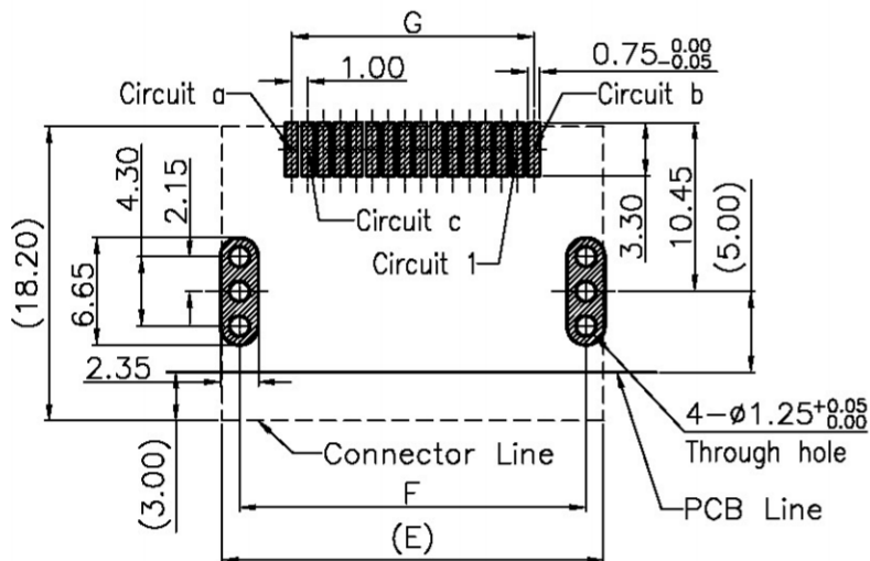
Recommended P.C.B Layout(T=1.6mm)
